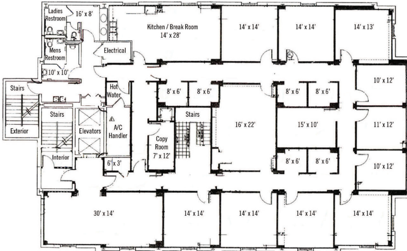
4th FLOOR
