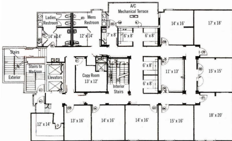
5th FLOOR
