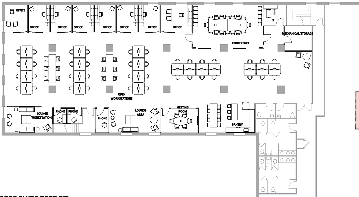
1 SPEC SUITE TEST FIT 3/32" = 1'-0"
