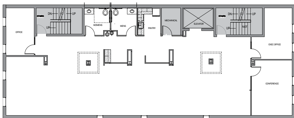
1 PARTITION PLAN 1/4"=1'-0"
